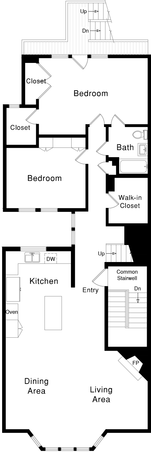
Main Floor
